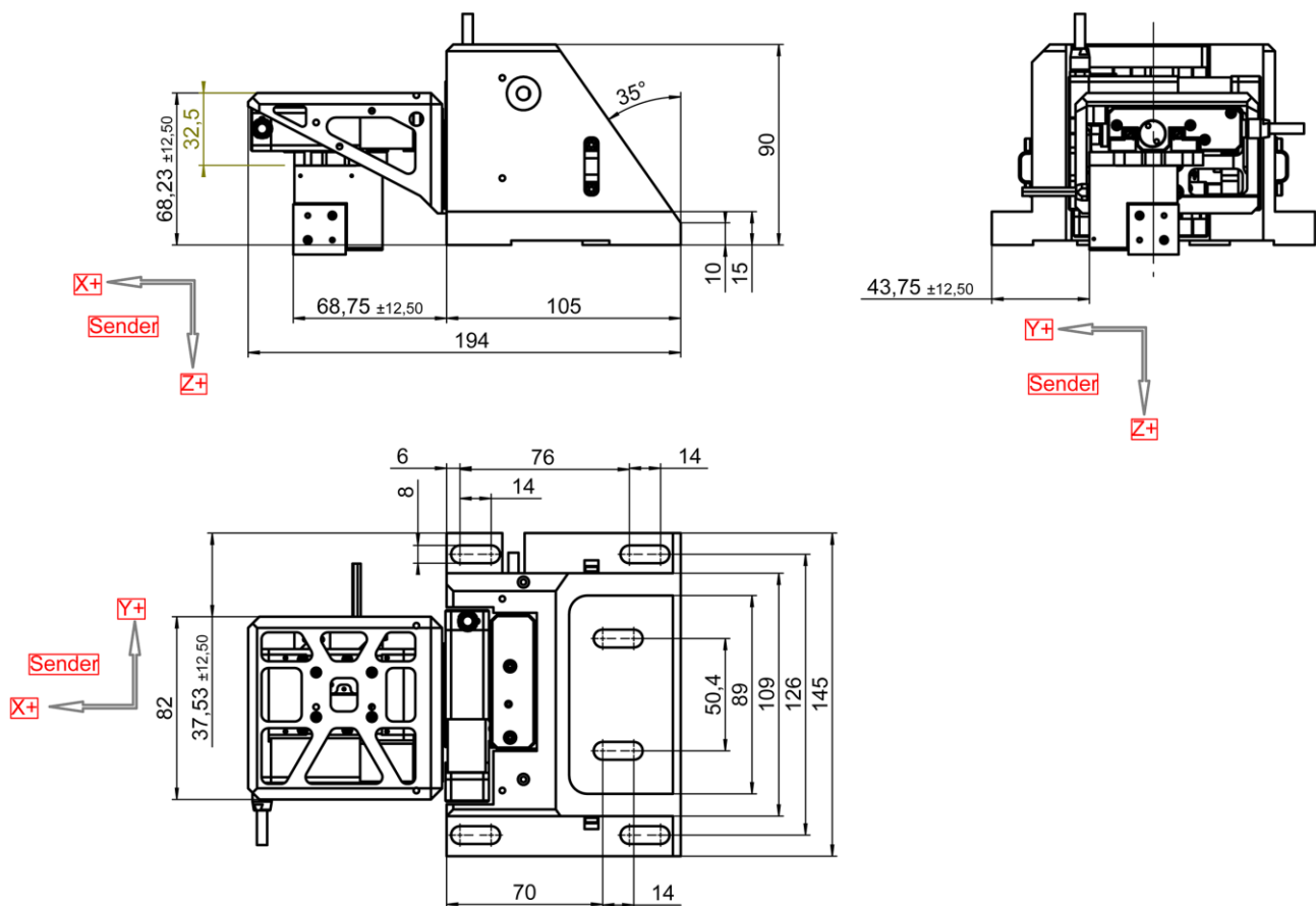
F-712.MA1, dimensions in mm
